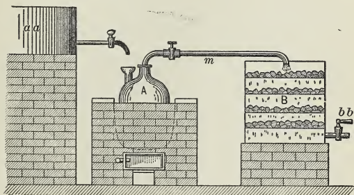
FIG. 25.—Würth's Apparatus.
